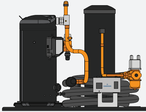
Scroll Water-Cooled Condensing
