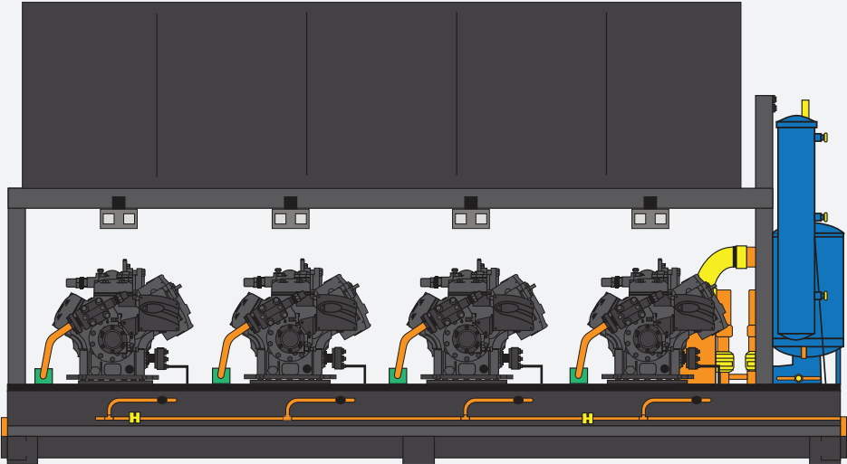
Copeland Semi-Hermetic Compressor
